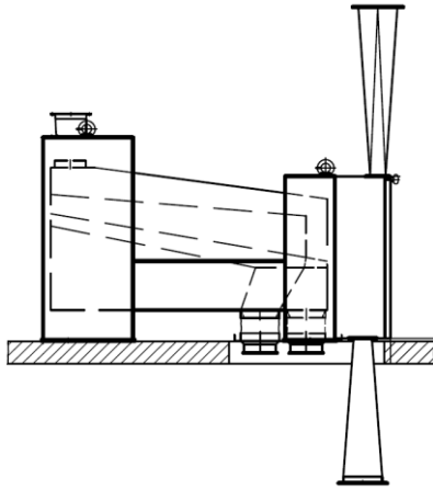
GrainPlus – without inlet aspiration
