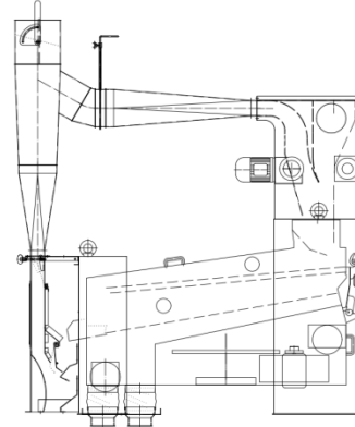
GrainPlus - with inlet aspiration
